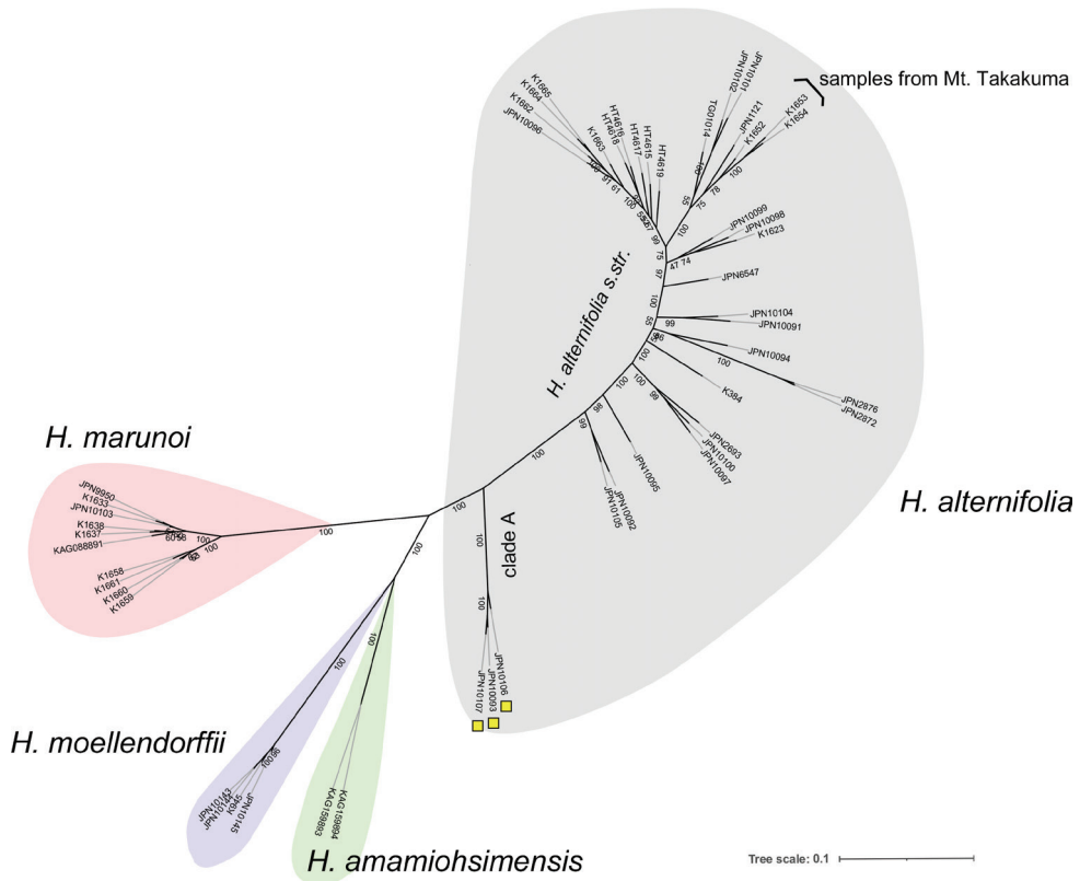
Figure 2. Molecular phylogenetic tree using MIG-seq data of 52 samples of Hydrangea sect. Cardiantora . Bootstrap values are shown on the internodes.
